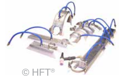
Argweld® Weld Trailing Shields®
